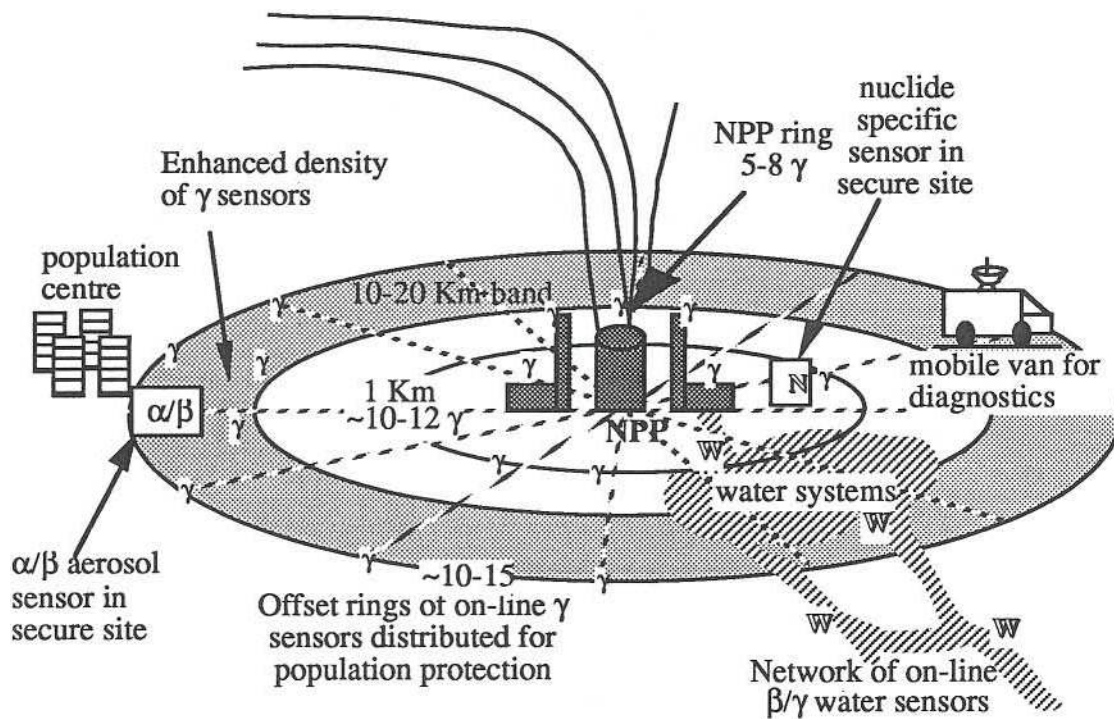
Figure 1: Outline Pilot Sensor Arrangement
